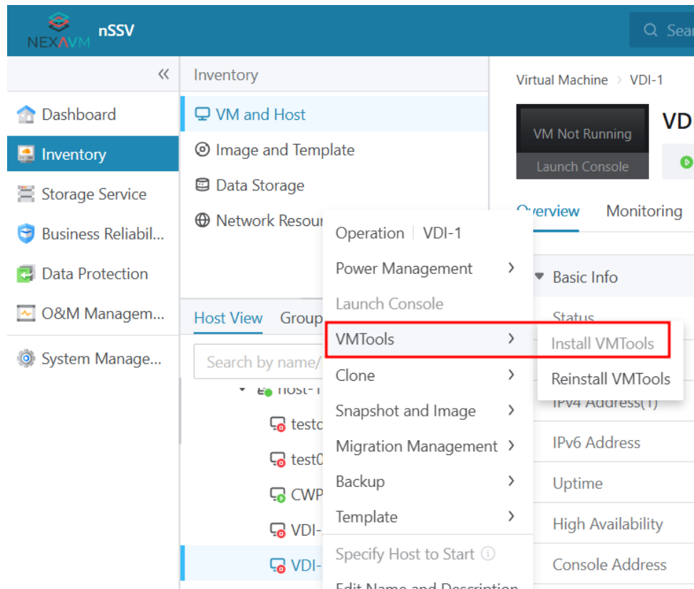
Figure 4: VMTools Installation
