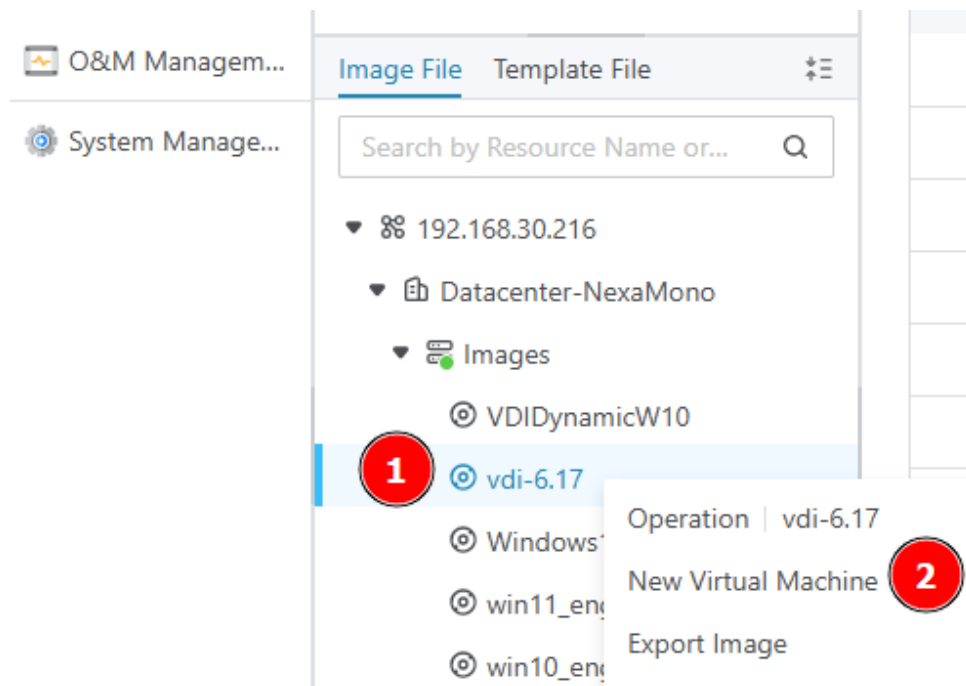
Figure 2: Create VM
