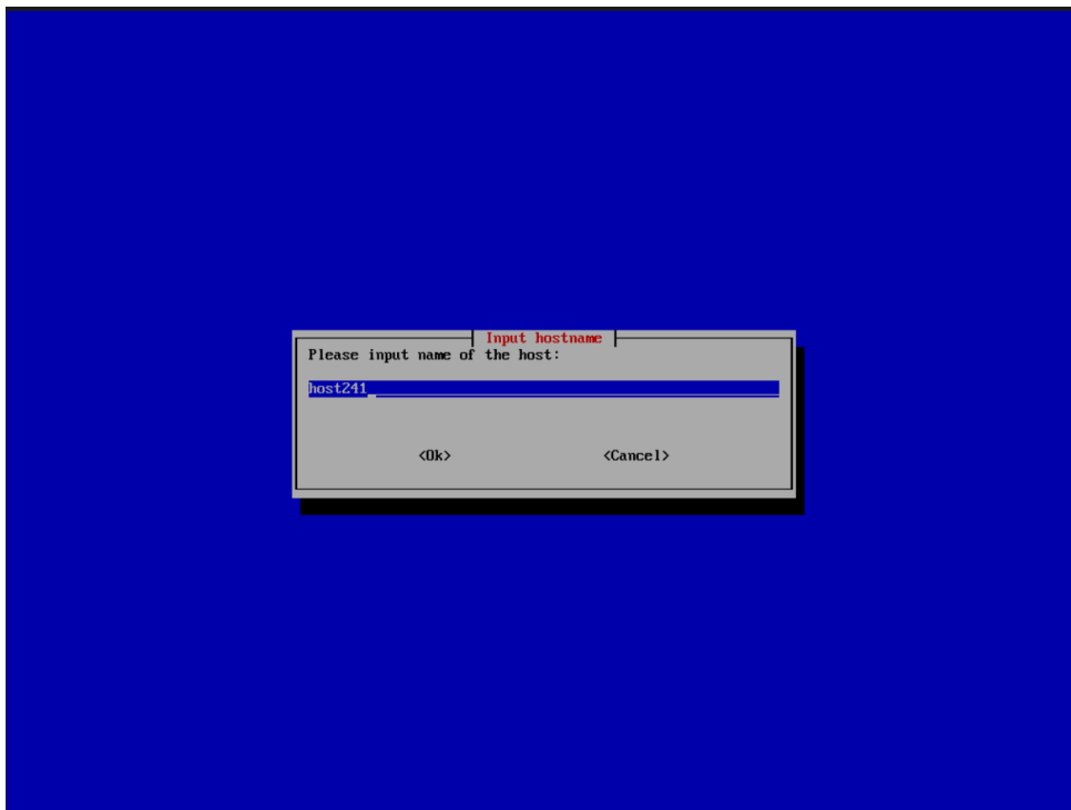
Figure 5: Slave VM
