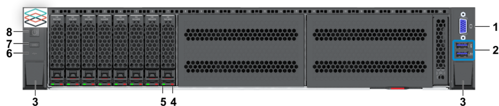
Figure 2-3 Front Panel with Eight Vertical Disk Slots
