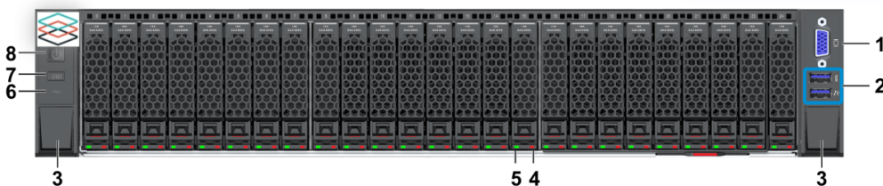
Figure 2-6 Front Panel with Twenty-Five Vertical Disk Slots
