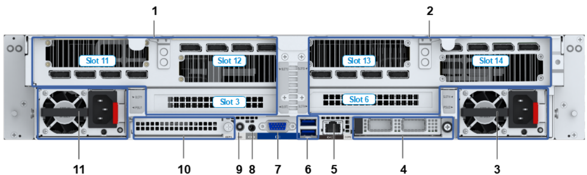
Figure 2-9 Rear Panel of the 4-GPU Model
