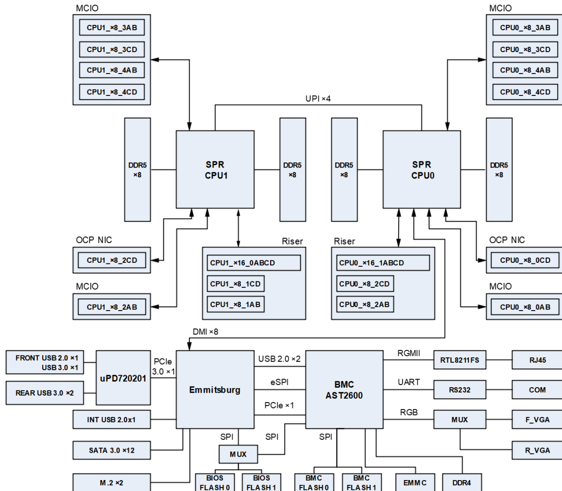
Figure 3-3 Logical Structure
