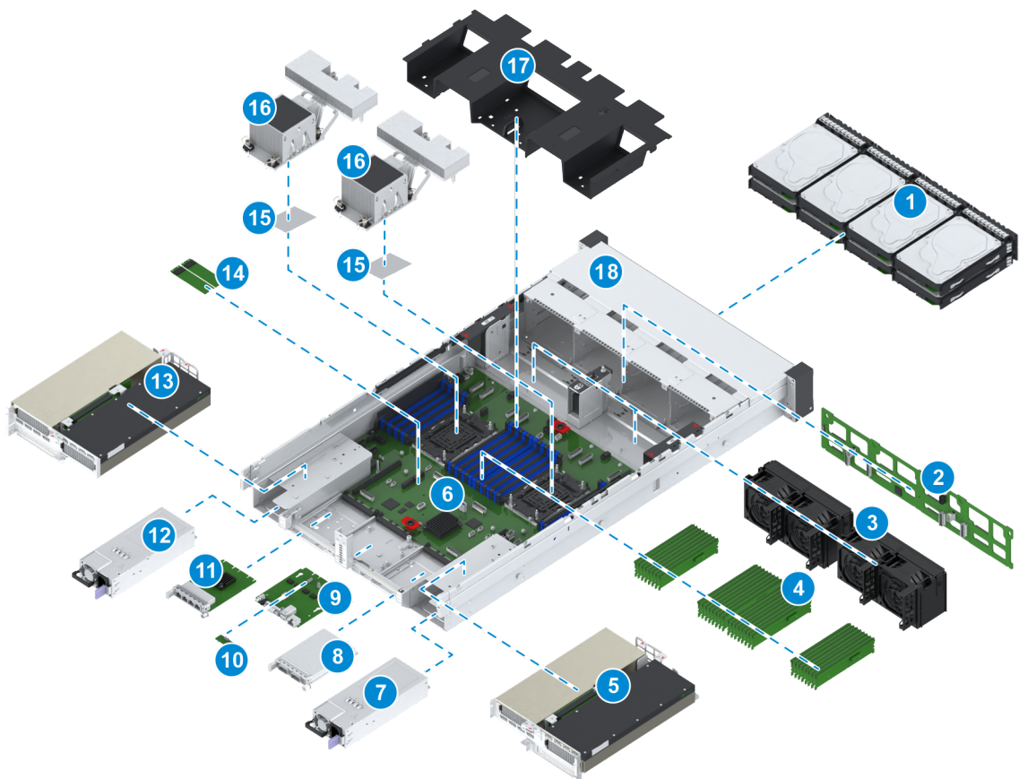
Figure 3-2 Internal Layout
