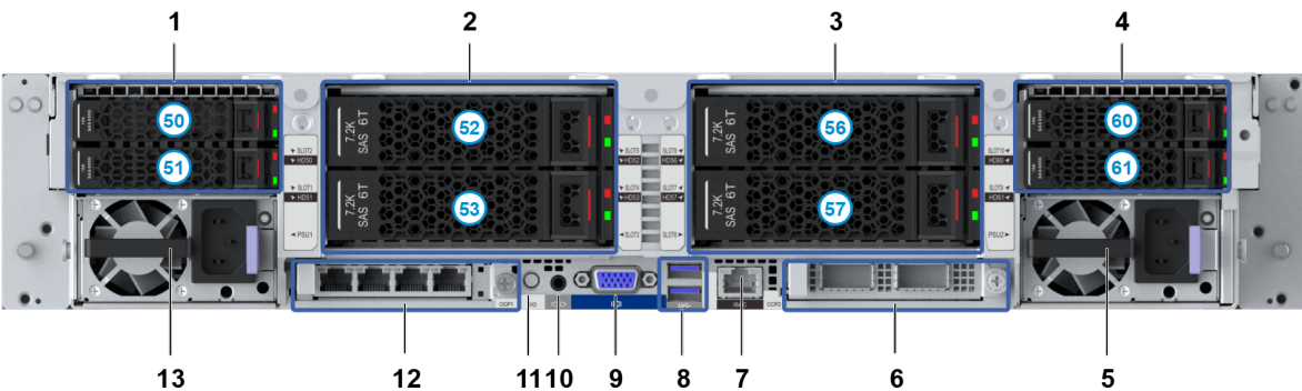
Figure 2-8 Rear Panel with Hard Disk Slots Only
