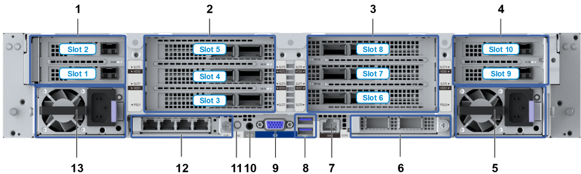
Figure 2-7 Rear Panel with PCIe Slots Only
