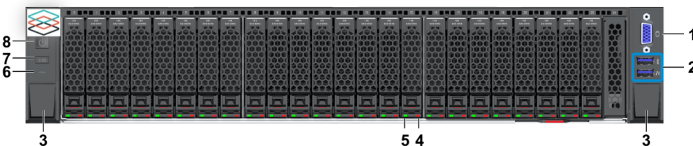
Figure 2-5 Front Panel with Twenty-Four Vertical Disk Slots
