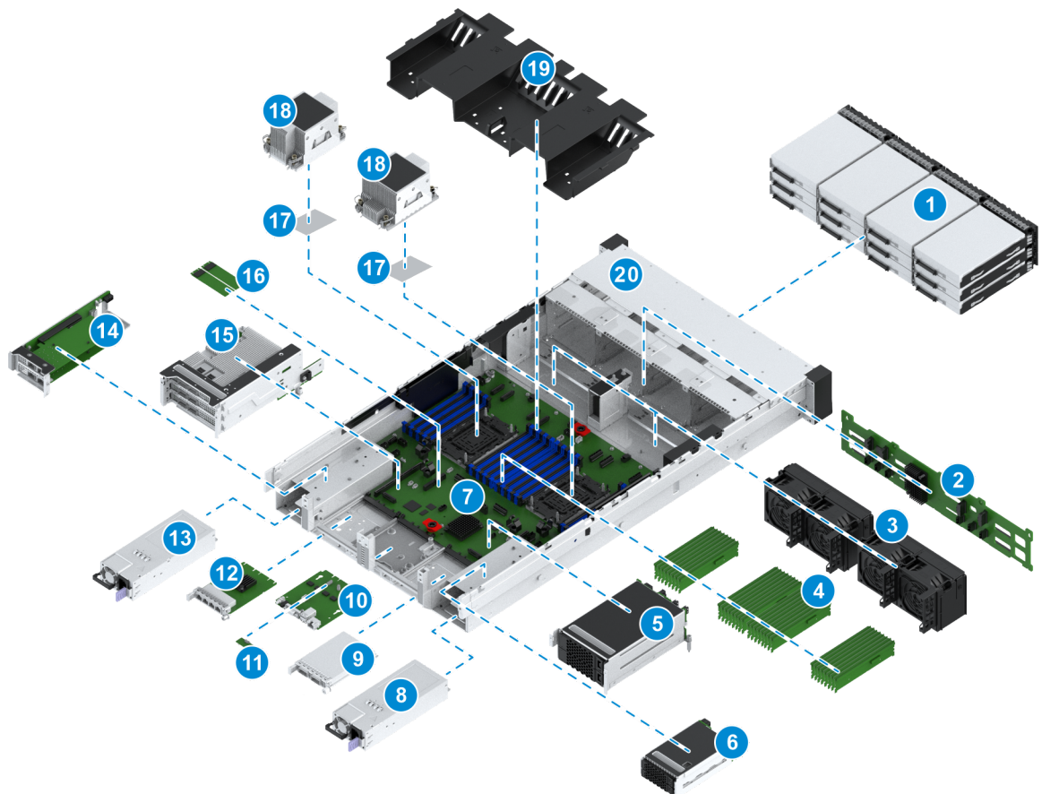
Figure 3-1 Internal Layout
