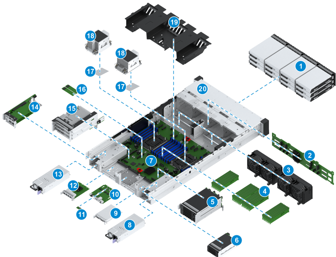
Figure 3-1 Internal Layout
