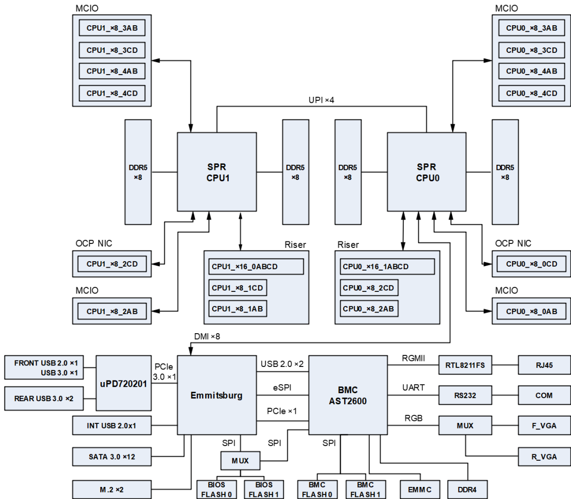
Figure 3-3 Logical Structure
