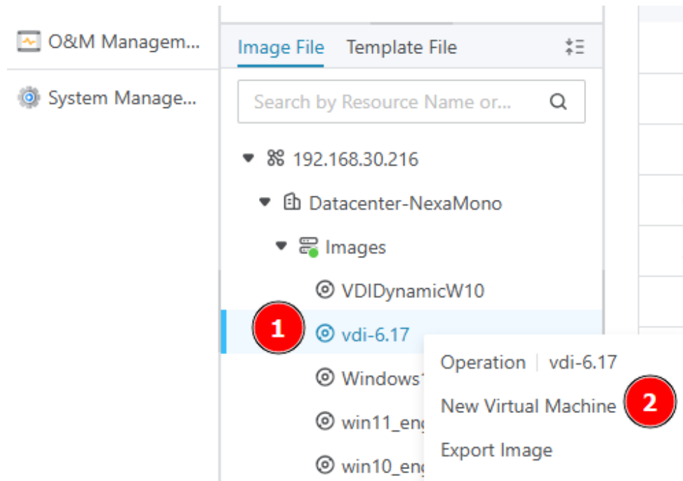
Figure 2: Create VM
