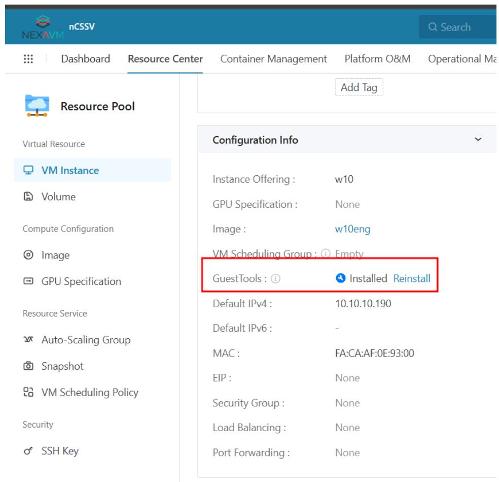
Figure 4: VMTools Installation
