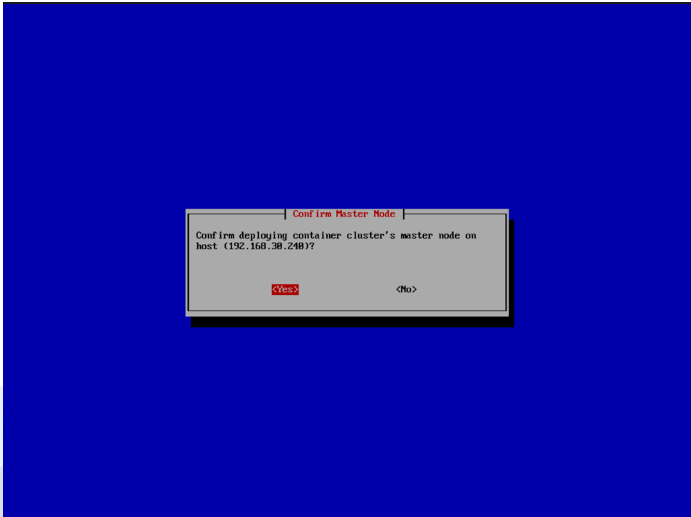
Figure 7: Master VM
