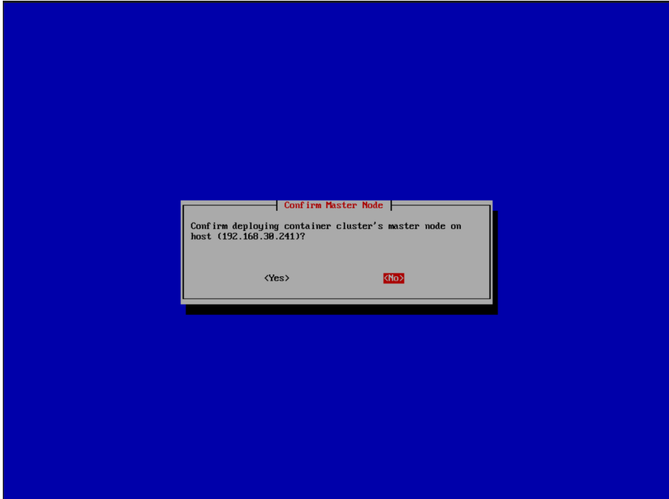
Figure 6: Slave VM
