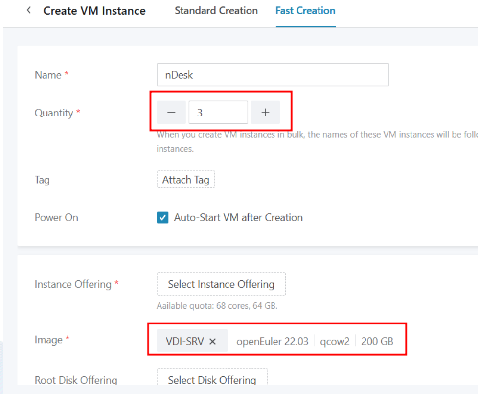
Figure 3: Create VM
