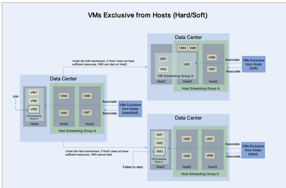
Figure 9-4: VMs Exclusive from Hosts (Hard/Soft)
